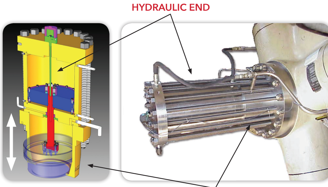
ADDITIONAL CLEARANCE END
